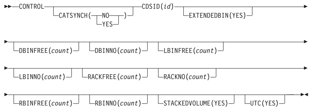
Figure 153. EDGUTIL SYSIN Commands
