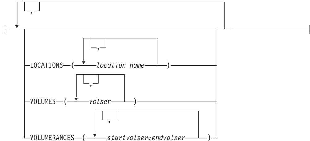
Figure 126. EDGHSKP SYSIN File
